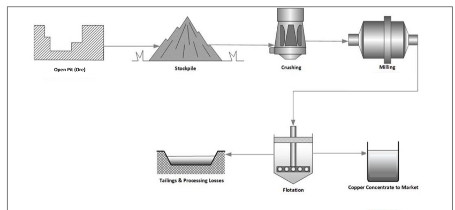
FIG 2: Process Flow Diagram
